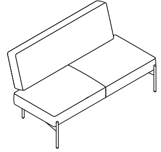
TI2PN L: 1480 P: 780 HT: 810 HS: 420
