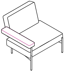
TI1DN L: 930 P: 830 HT: 810 HS: 420 HB: 610
