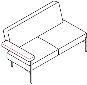
TI2DN L: 1560 P: 830 HT: 810 HS: 420 HB: 610
