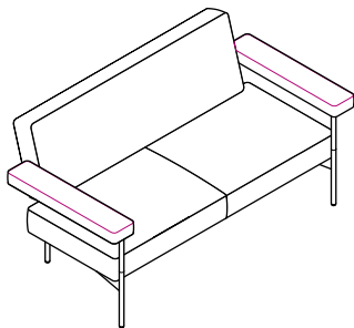
TI2BN L: 1640 P: 830 HT: 810 HS: 420 HB: 610
